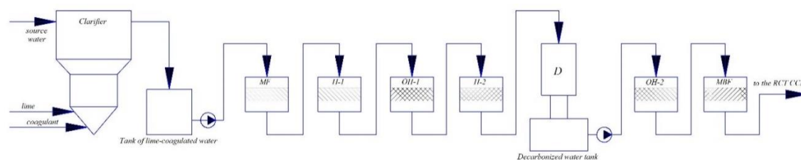
Fig. 1. «Traditional» preparation scheme for deeply desalinated water: MF – mechanical filter, H-1 and H-2 – H-cationic first stage filters, OH-1 and OH-2– OH-anionic first stage filters, D – decarbonizer, MBF – mixed-action filter, RCT – tank of spare condensate
